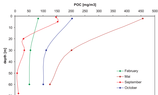
Fig. 3. Measured particulate organic carbon concentrations [ \text{mgC m}^{-3} ]
