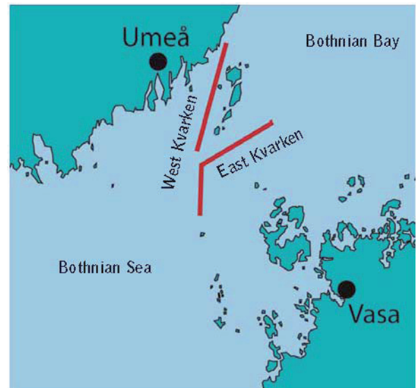
Fig. 2. Two channels carry water into and out of Bothnian Bay (Western and Eastern Kvark straits), passing on both sides of the Holm Islands. The maximum depth of the channels is 25 meters. Measurements were made here to learn more about water exchange between the two basins.
