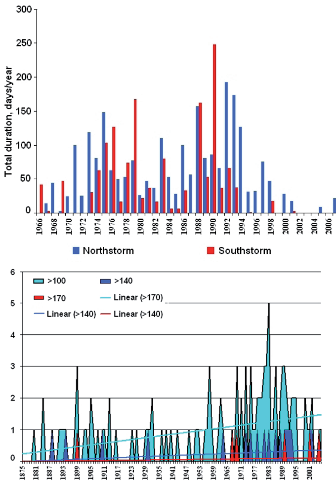
Figure 2. Duration of northern and southern storms (24-hour speed > 8 m/s) in the south of the Gulf of Riga for the period 1966-2006 (upper panel), and changes in frequency of extreme water levels in Lielupe River mouth for the period 1875-2006 (lower panel).
