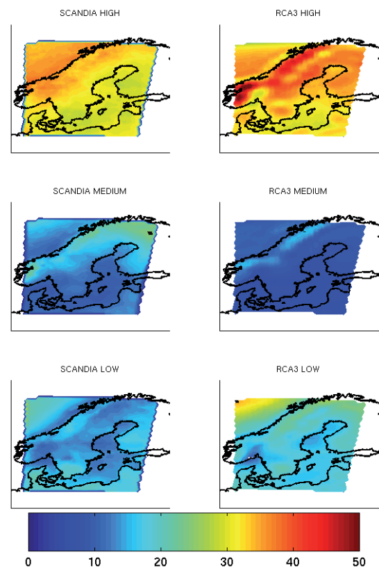
Figure 1. Annual mean (excluding Winter) 1991-2000 of the high-level (upper panels), medium-level (middle panels) and low-level (lower panels) cloud cover contribution to the satellite-viewed total cloud cover (%) for SCANDIA compared with RCA3 simulations. Results are shown after applying optical thickness cutoff on RCA3 results.
