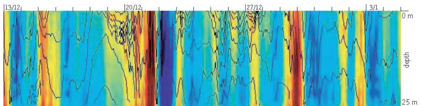
Fig. 3 Flow rates, measured hourly, in the West Kvark Strait at the end of 2004. Time is plotted on the horizontal scale, depth on the vertical scale. The currents range between northerly (red) and southerly (blue), and flow at up to 0.5 m/s. Note the rapid changes in flow direction, and the consistency of the currents all the way from the surface to the bottom. Thin lines indicate density differences (from Green, Liljebladh and Omstedt 2006)
