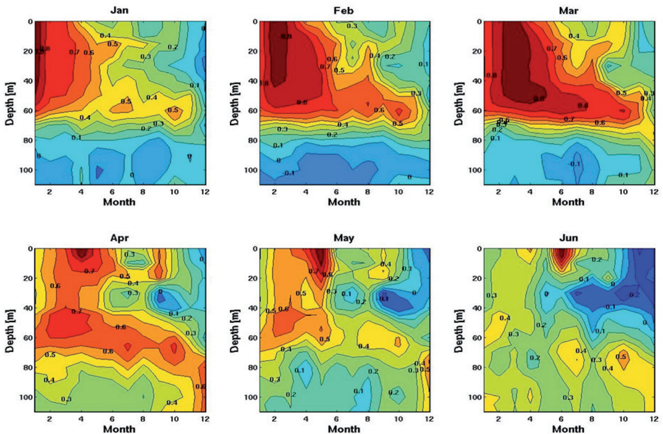
Fig. 5. Correlation coefficients between January and June SST and deeper water mass temperatures for all months at ICES SD 26 (Gdansk Deep). The high correlation coefficients (in red) demonstrate a strong linkage between surface and mid water temperatures.
