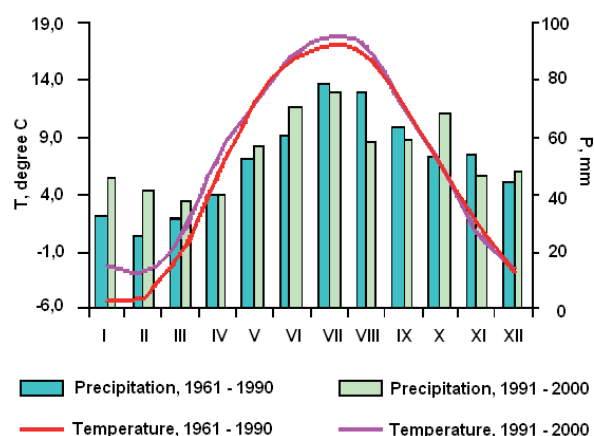
Figure 1. Regional data series of temperature (line) and precipitation (column) for the reference period 1961-1990 and the last decade
