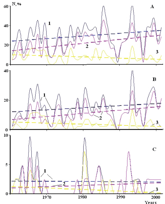
Fig. 1. Multi-year variability of the area (in % of total area) where snow storage in December (A) does not exceed half of the standard deviation, (B) exceeds the standard deviation, and (C) exceeds twice the standard deviation. – (curve 1, blue) represents the studied territory on the whole, (curve 2, pink) represents the northern part of the East European Plain, and (curve 3, yellow) stands for the Scandinavian peninsula. Dotted lines represent the respective linear trends.
