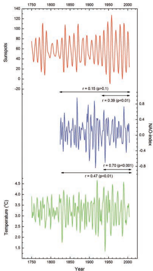
Fig. 1. Sub-series correlations ( r ), with Monte Carlo based statistical significance ( p ) of the correlations, calculated between the band-pass filtered records of sunspot numbers (Waldmeier 1961), the NAO-index (Jones et al. 1997) of spring season and reconstructed spring temperatures (Holopainen et al. 2009), calculated for the period 1825-2004 (long arrow) and 1935-2004 (short arrow).
