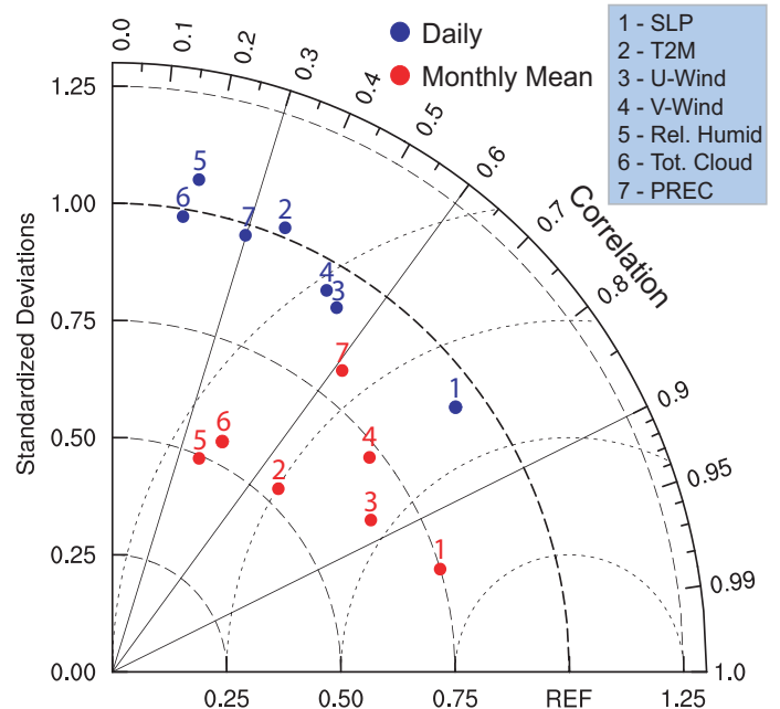
Figure 1. Taylor diagram for January showing reconstruction skills of mean field correlation and ratio of variance \text{var}(\text{REC})/\text{var}(\text{RCAO}) for the period 1958-2007 on daily and monthly scale
