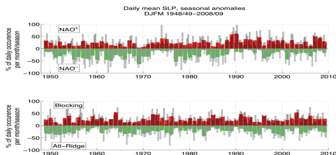
Figure 4. Time history of occurrence of the NAO, Atlantic Ridge and Blocking regimes over the period 1949-2008. Vertical bars give the number of daily occurrence per season (filled bars) / per month (contoured bars) during winter (DJFM) for the given regime.
