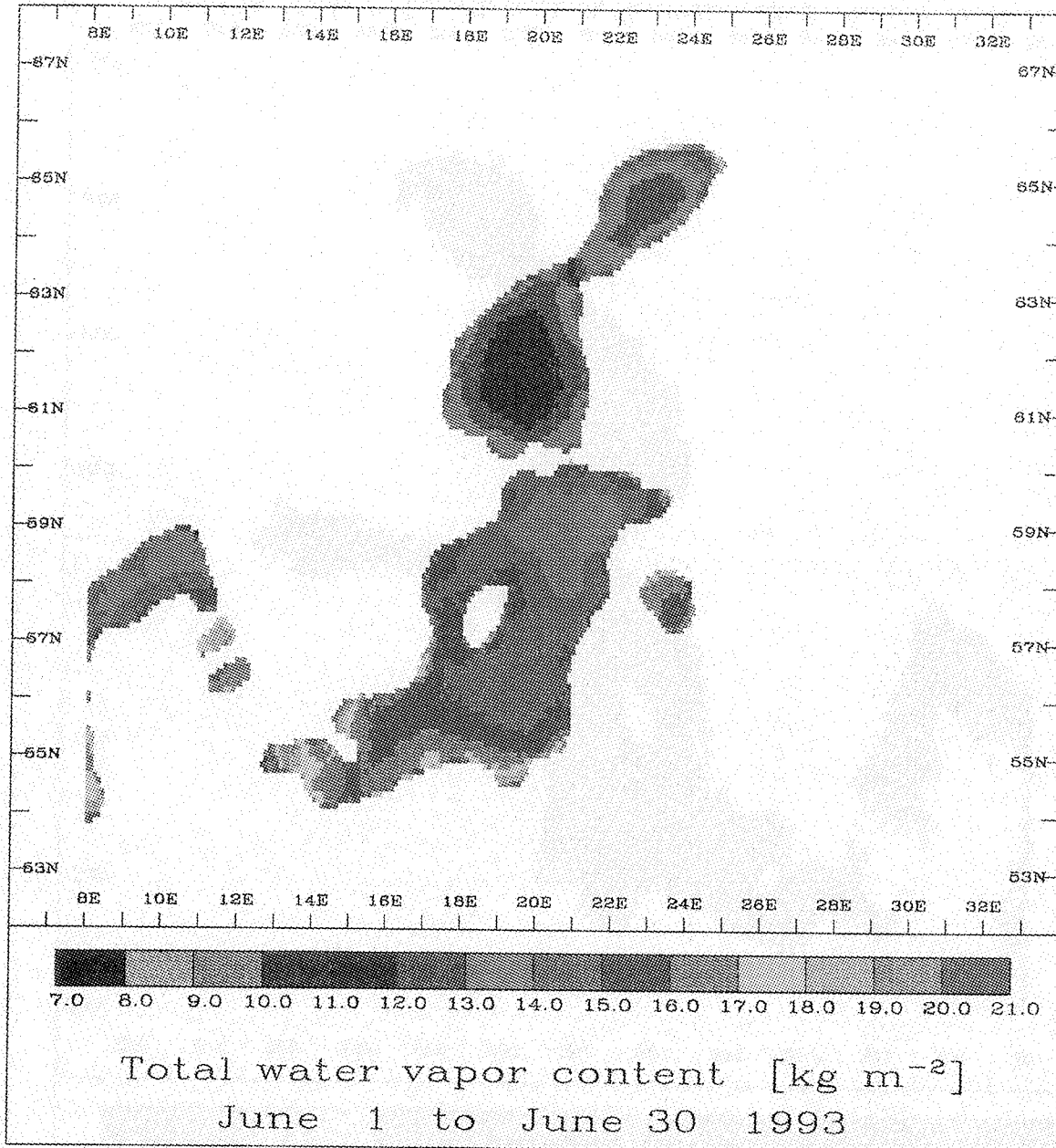
Figure 1: Monthly mean total water vapour content for June 1993, estimated with the neural network based algorithm from Jung (1996). Land influences inside the half power beam width are removed.
