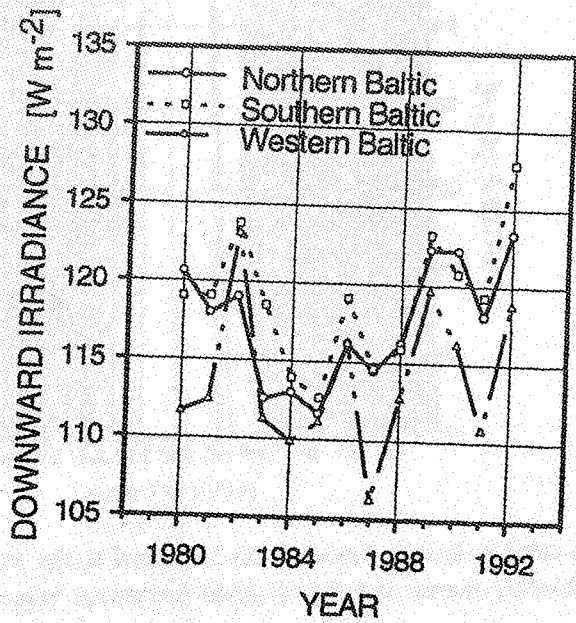
Figure 1 (left): Interannual variations in the annual mean solar radiation fluxes at the Northern, the Southern and the Western Baltic Proper during 1980 to 1992.
