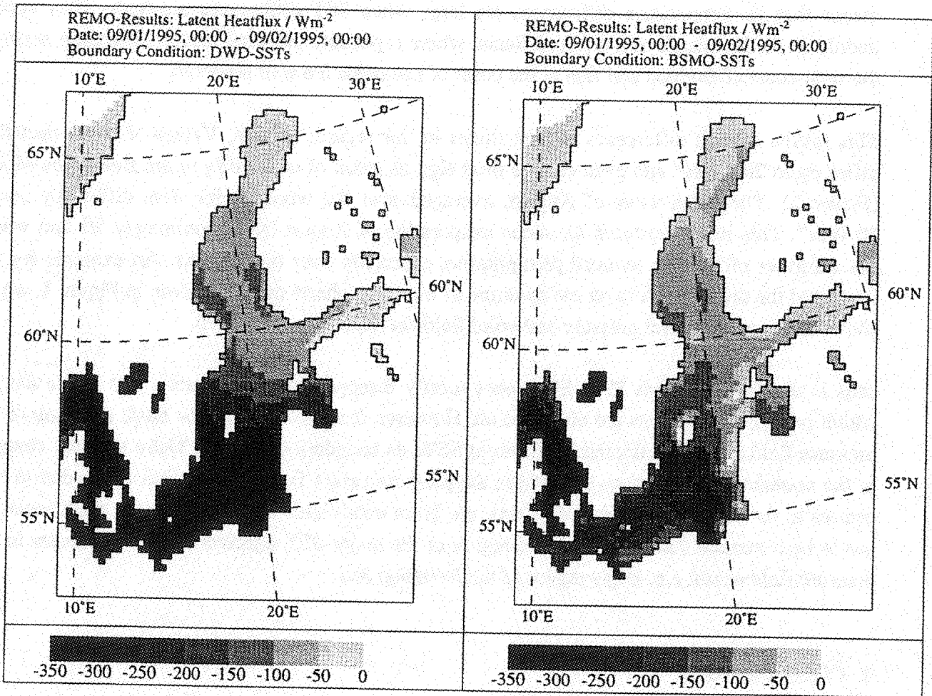
Figure 2: Mean latent heatflux, 09/01/1995, 00:00 - 09/02/1995, 00:00; left: SSTs from DWD analyses as boundary condition, right: SSTs from BSMO as boundary condition.
