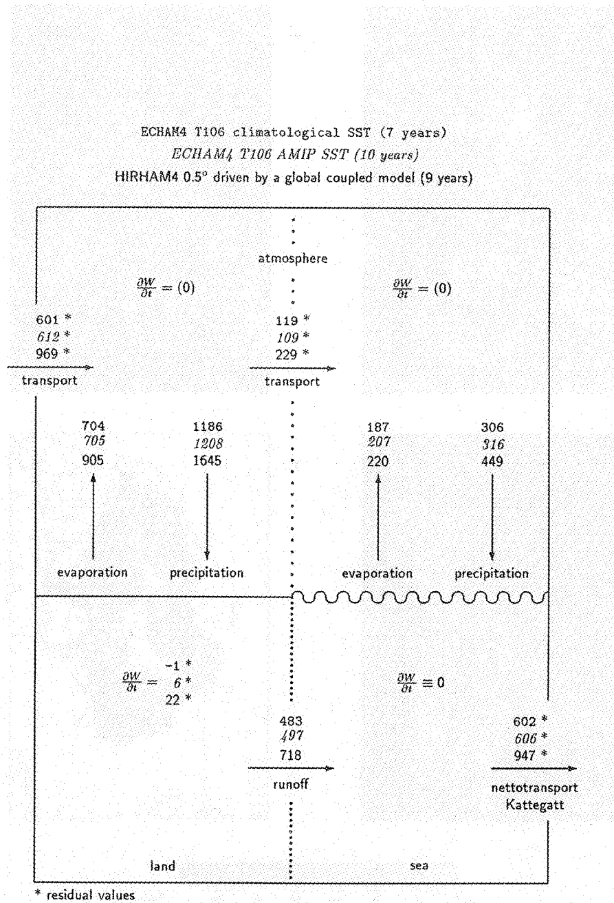
Figure 4: Water budget for Baltic Sea drainage basin [km³/year]
