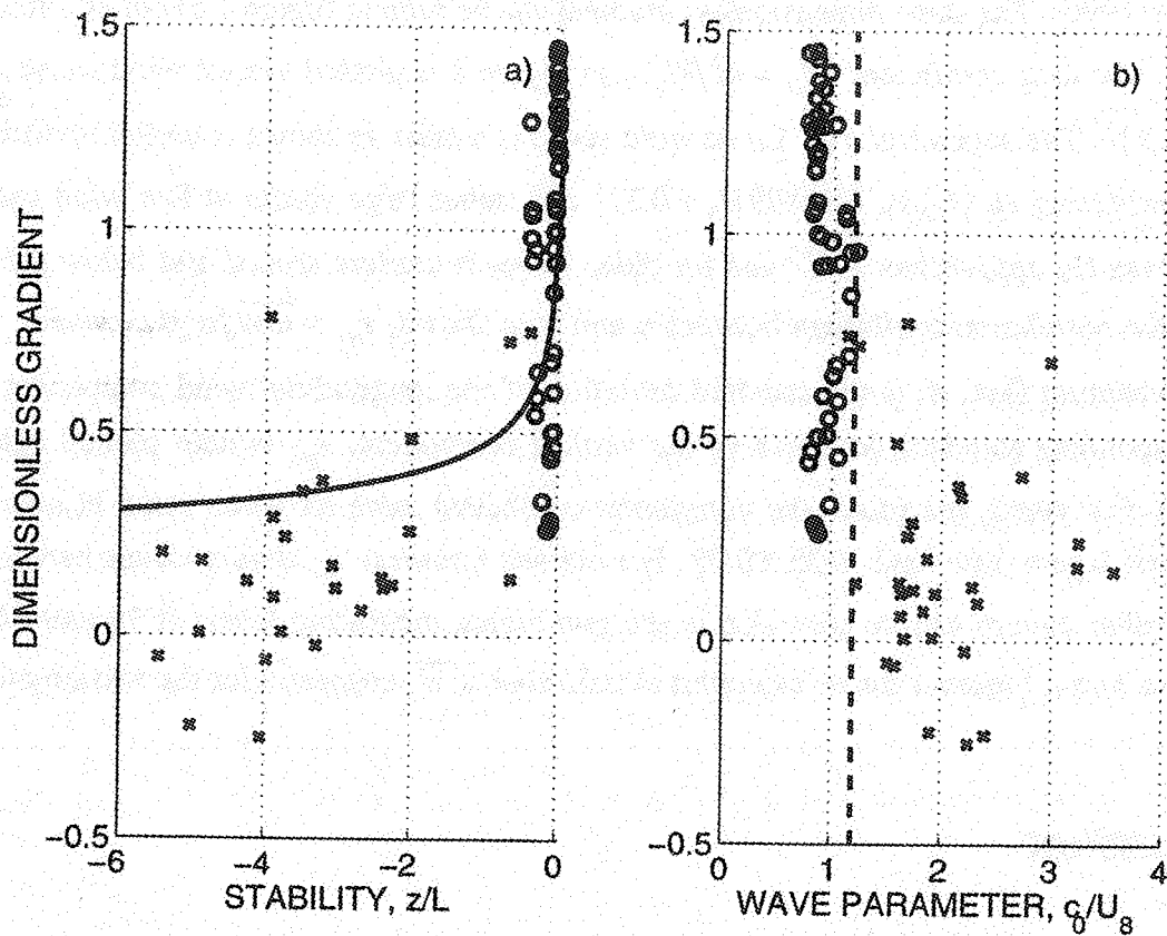
Figure 1: Dimensionless gradient ( \partial U/\partial z * zk/u_* ) versus a) stability parameter z/L , b) wave parameter c_0/U_8
