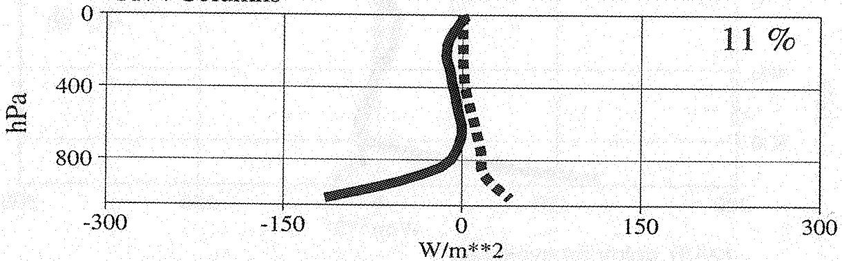
Figure 2: Averaged profiles for objectively sorted columns for three different types; both convective heat and rain fluxes shown. Relative frequency given in upper right corner. Valid from 18 UTC - 6 UTC. Dataset 32 x 32 columns over Europe for first day of each month for 1991, using ERA data.
