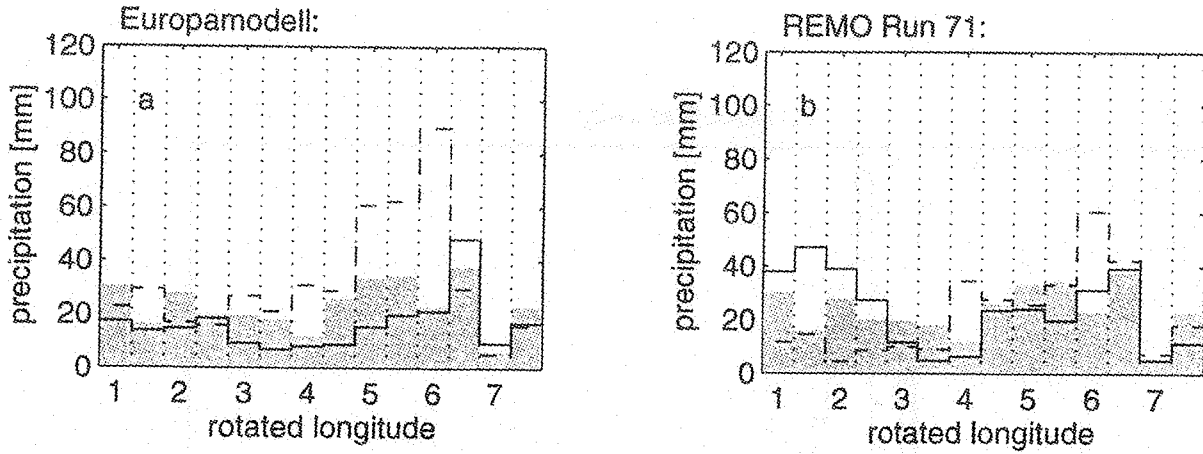
Figure 3: Cumulated precipitation along the ship's tracks. In situ measurements (shaded columns), convective portion (dashed line) and stratiform portion of modelled precipitation (solid line) are shown.
