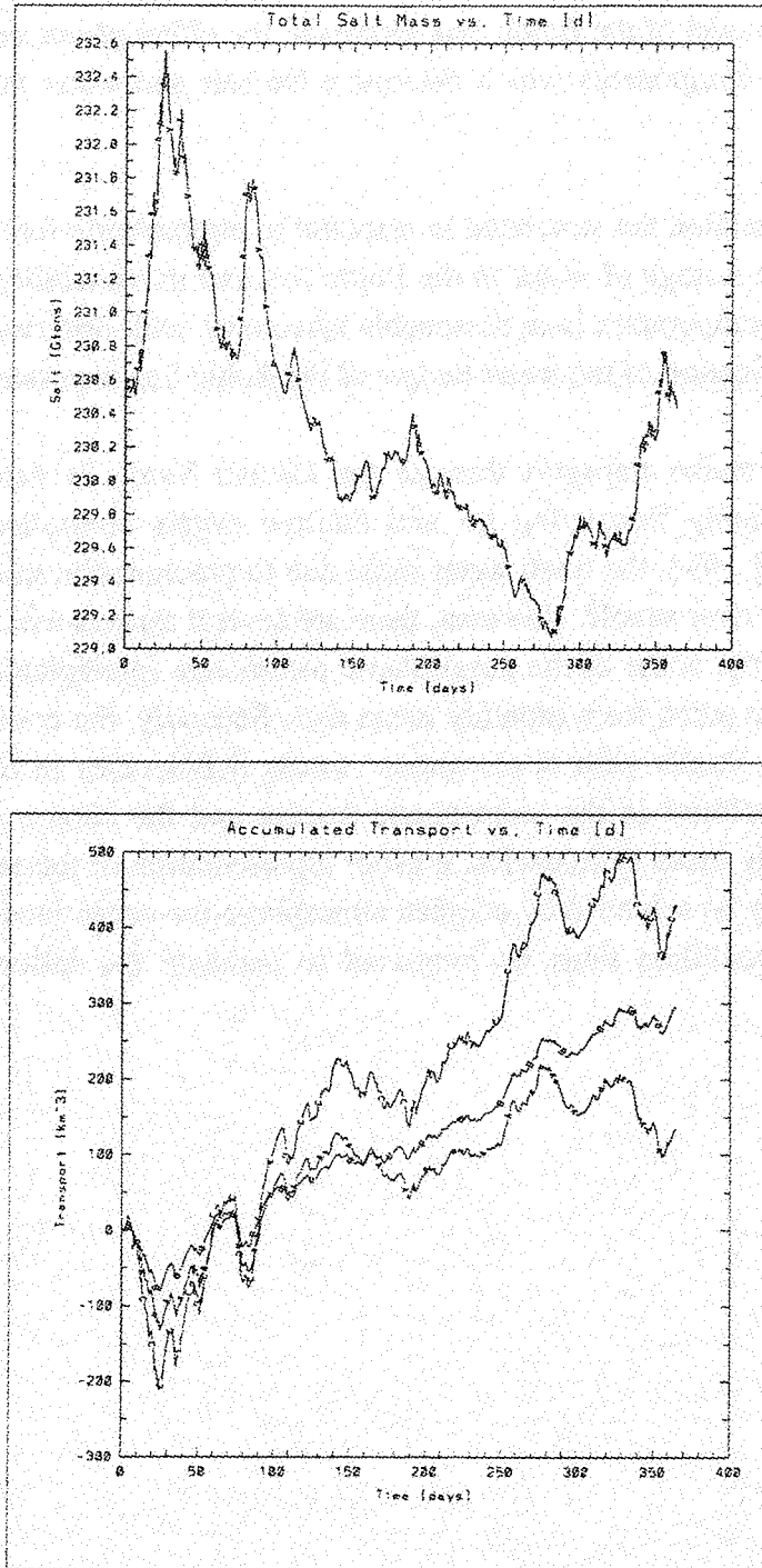
Figure 4: Accumulated volume transport and total salt content of the Baltic Sea for 1993, lower panel: A, B and C denote the transport through Sound, Great Belt and Belt Sea (sum of A and B), respectively.
