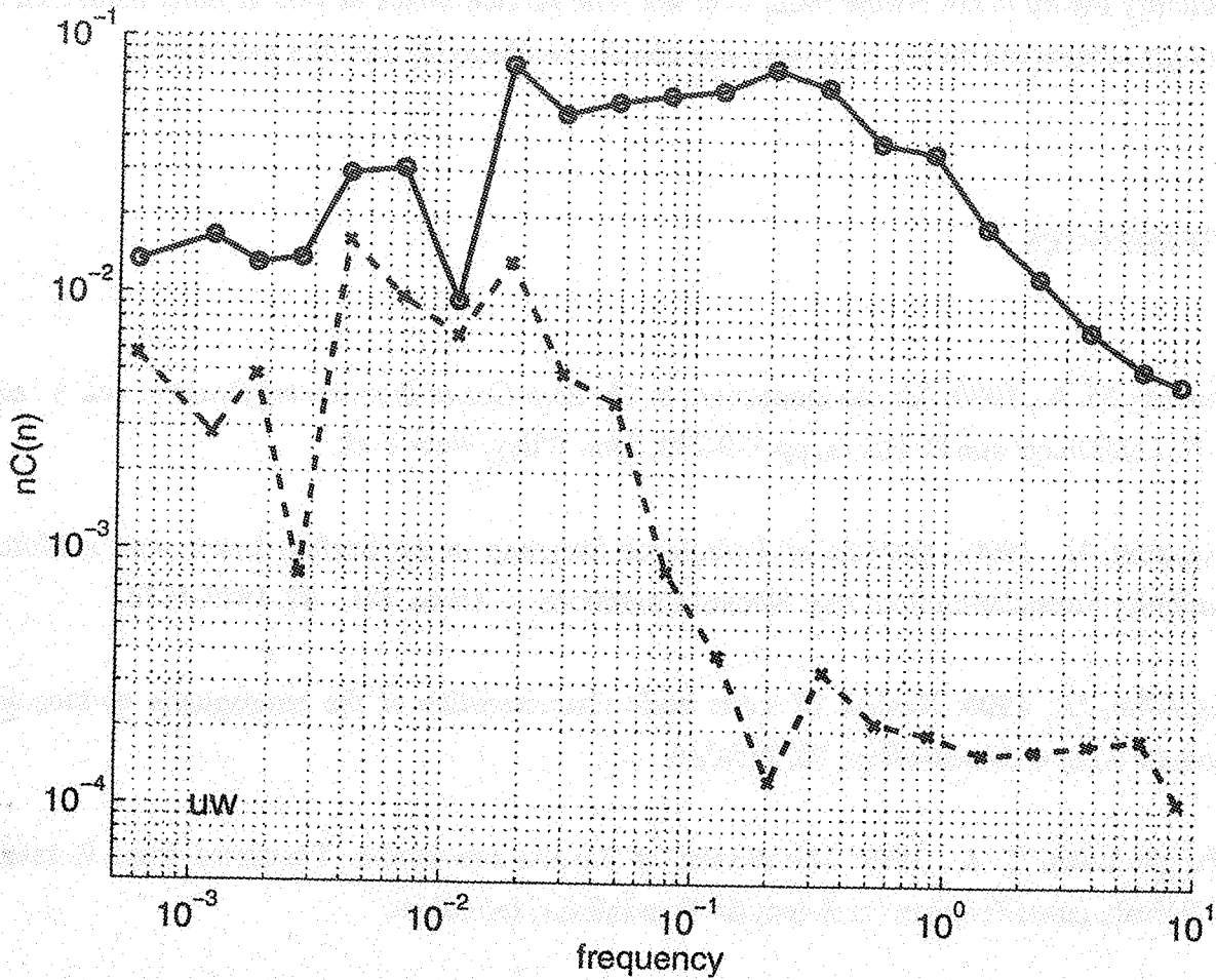
Figure 4: The cospectrum of vertical transport of momentum as a function of frequency.
