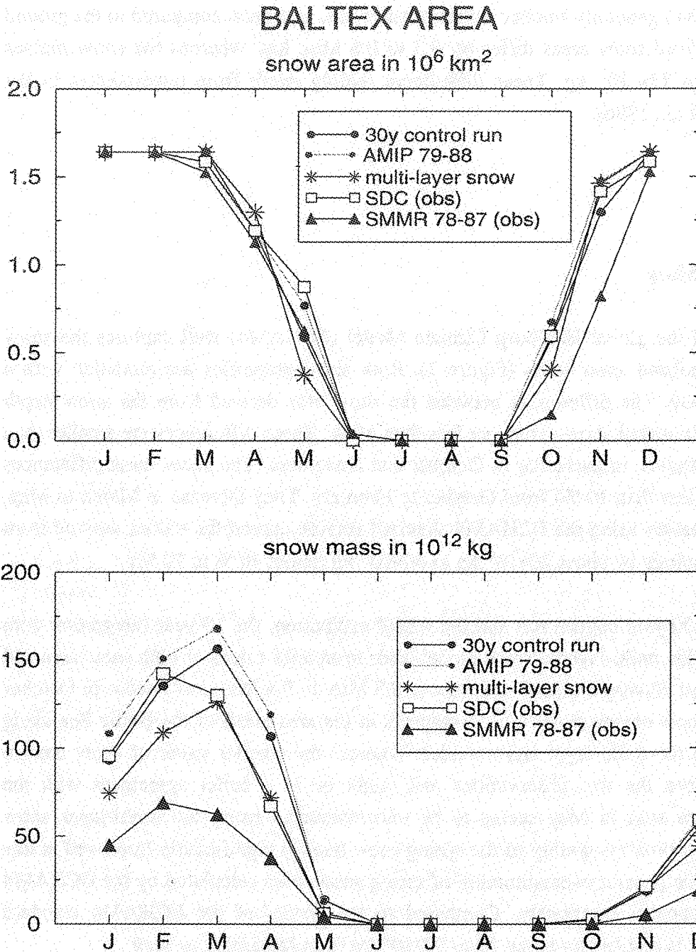
Fig.1: Mean annual cycle of snow area and mass derived from ECHAM4 climate simulations and observations. Simulation results are shown for the 30y control run, the AMIP period (1979-88) and the case that a multi-layer snow model was implemented into ECHAM4. The calculations are compared with values derived from ground observations (Snow Depth Climatology, revised version of Foster and Davy, 1988) and satellite data for 1978-87 (SMMR, Foster et al., 1996).
