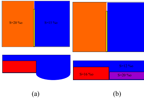
Figure 4. Model area and initial salinity distribution
