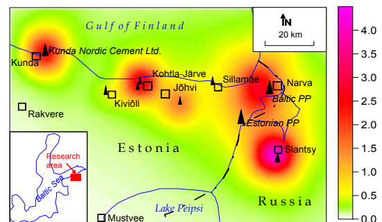
Figure 1. Cumulative deposition load of alkaline particles during 1960 – 2000, kg/m 2 . Black triangles mark the emission sources.
