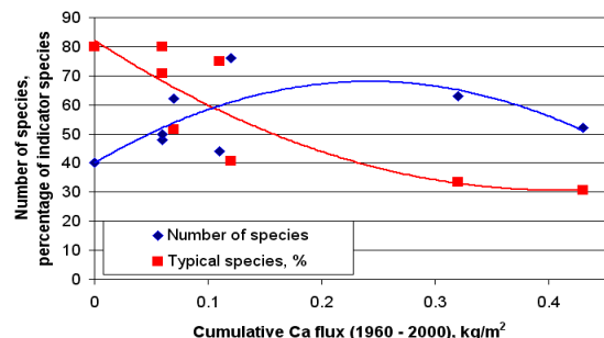
Figure 3. Total number of species and percentage of typical species at 100 m 2 squares of different bogs (ridge-hollow bog, in 2000 – 2001) vs. calculated cumulative deposition flux of calcium.
