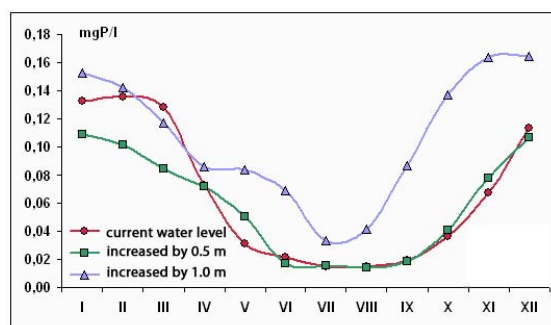
Figure 4. Total phosphorous concentration in the Lake Zuvintas at different water levels
