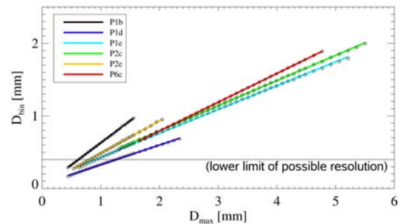
Figure 1. Simulated ice crystals
