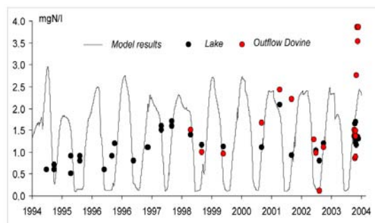
Figure 1. Calculated with PCLake and measured total nitrogen concentrations in the Lake Zuvintas and its outflow Doveine.
