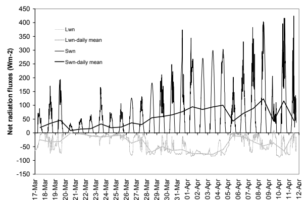
Figure 2. Surface longwave radiation budget L_n (10-minute values and daily means) and shortwave budget S_n (10-minute values and daily means) during the measurement campaign
