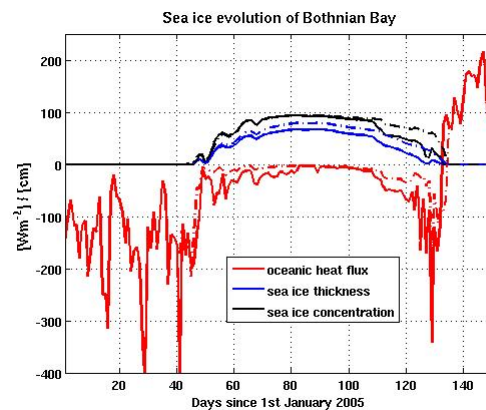
Figure 1. Simulated sea ice evolution and oceanic heat fluxes of the central Bothnian Bay, January to May 2005. Full lines represent the evolution affected by brine release, for broken lines, brine release was switched off.
