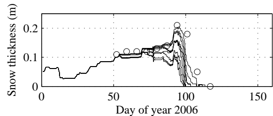
Figure 5. Modeled snow thickness with various albedo schemes incorporated into HIGHTSI. Dots are the measurement.
